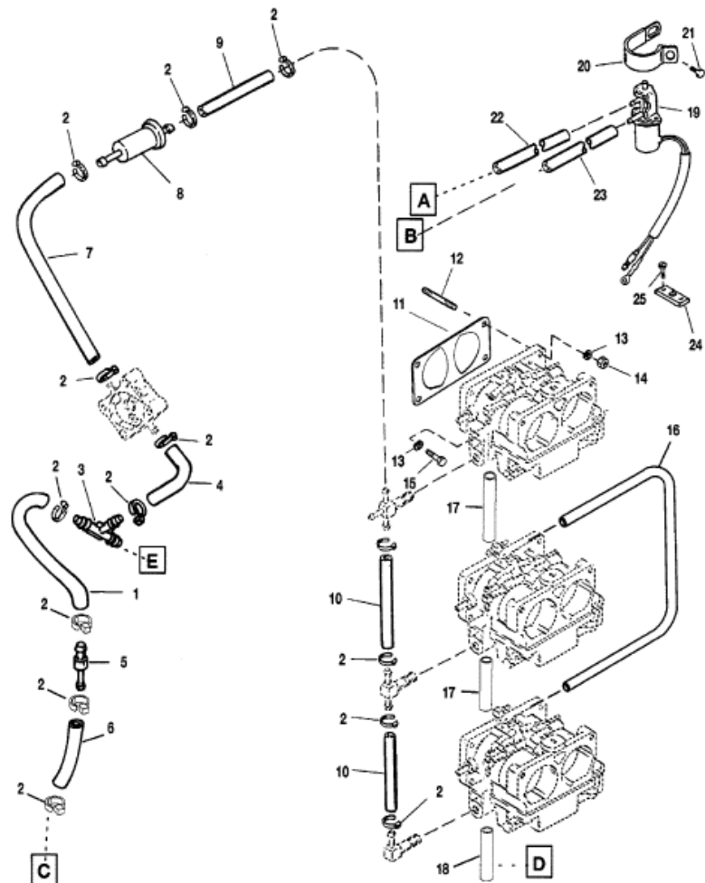
A= to top carb . . B = to middle carb . . . . C = to oil pump . D= to Cyl. Head . E = to primer bulb
